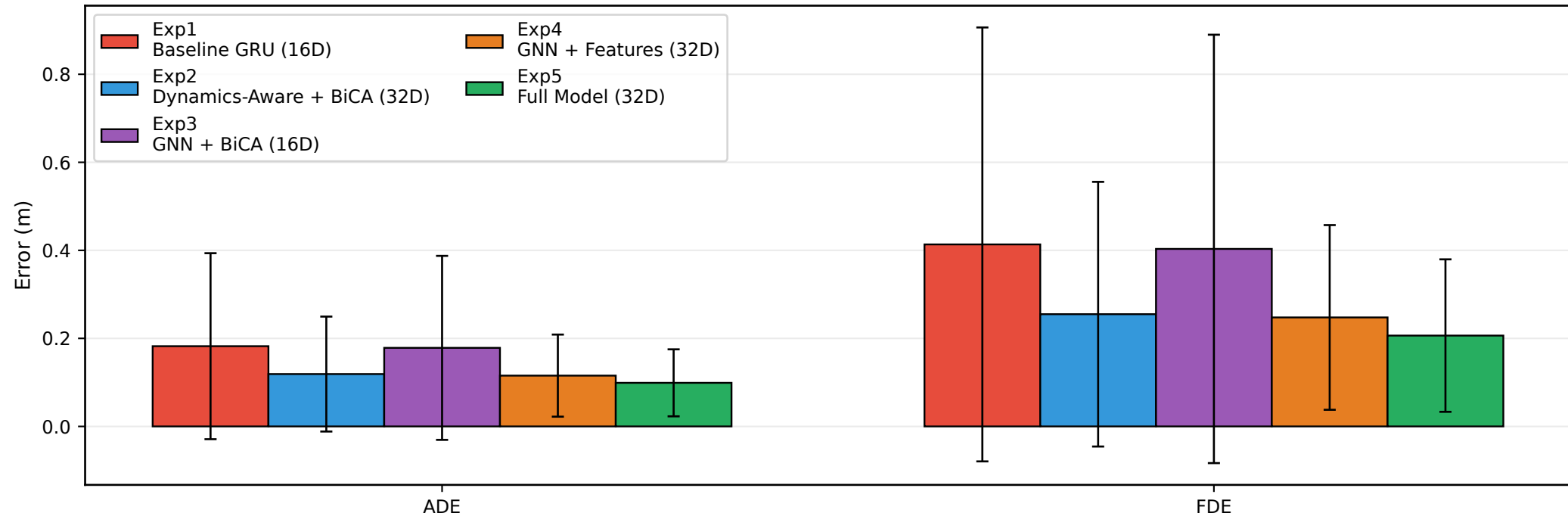
ADE/FDE comparison (mean \pm std)
